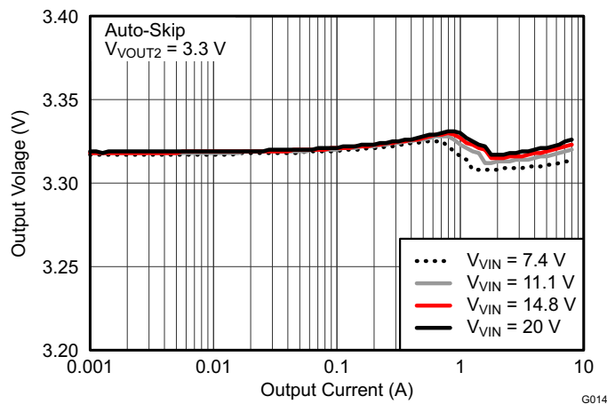
Figure 17. Load Regulation
