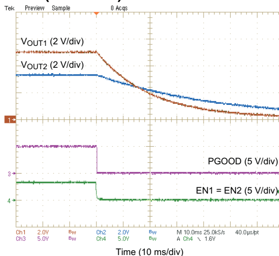
Figure 24. Output Discharge
